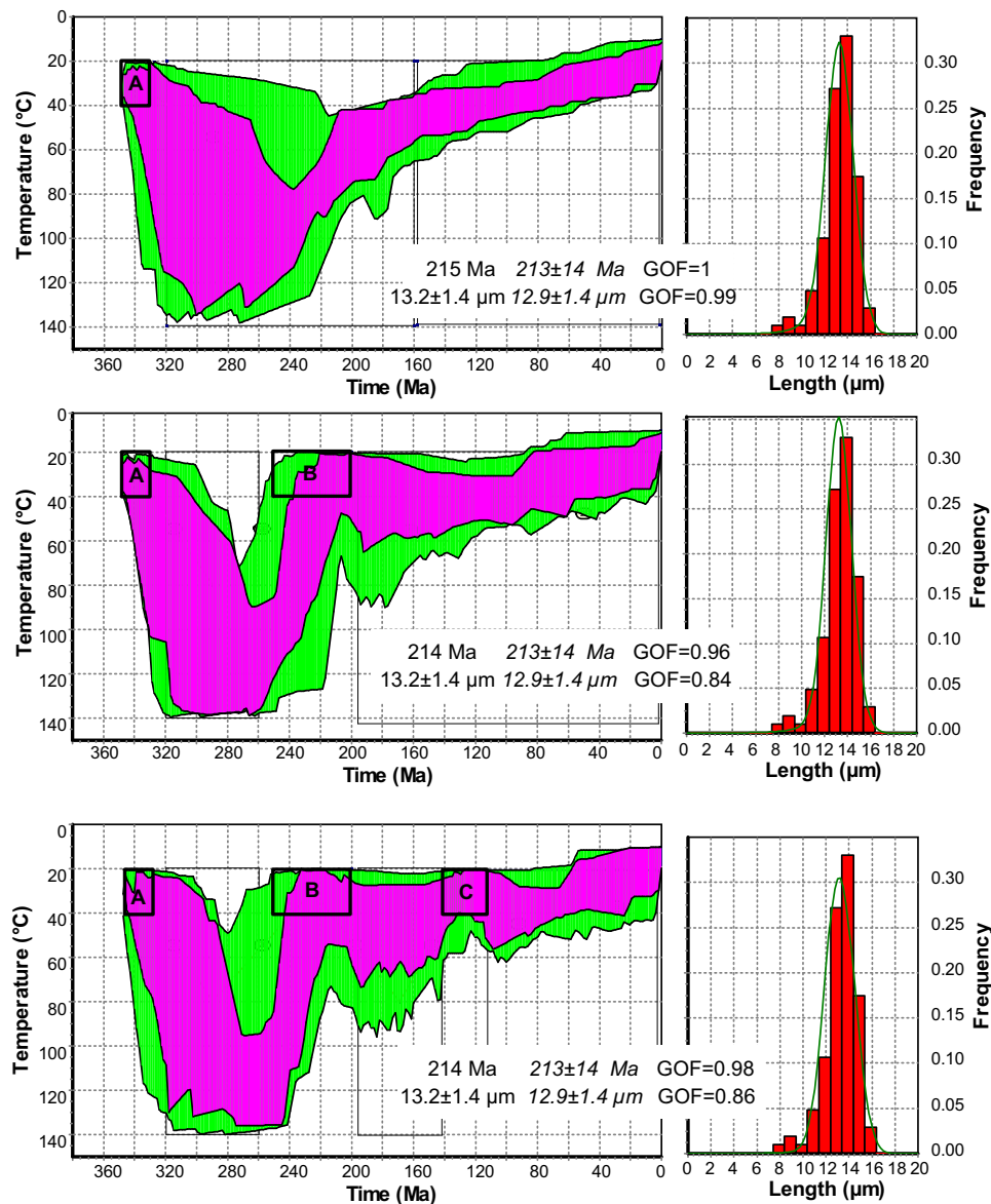
Fig. 5. Presentation for sample BEL28 of the different steps of the thermal modelling using AFTSolve ® . First step considers only that sample is at surface during the Visean and today. Second step introduced that sample is close to the surface (20–40 °C) during the Triassic. Last step considers that sample is close to the surface also during the Early Cretaceous. Numbers correspond to the measured (in italic) and modeled FT age and mean track length. GOF (goodness of fit) is an indicator of the match between the measured data and the data in agreement with the modeled thermal history (for perfect match, GOF = 1). Histograms correspond to the measured mean confined track length distributions; green lines attached to these histograms correspond to modeled distributions.
