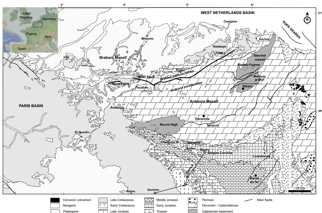
Fig. 1. Geological map of Northern France and Belgium (after De Vos et al. , 1992; Chantaine et al. , 2003). Boreholes used in Figure 8 are: (a) Blagny; (b) Sommathue; (c) Briquenay; (d) Grandpré; (e) Dontrien.
