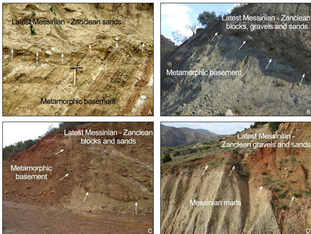
Fig. 9. Photographs of the Messinian Erosional Surface taken in four different outcrops located on both sides of the Alboran Sea. A, Guadario (Algesiras, Spain); B, El Túnel (Malaga, Spain); C, Tassafete (Oued Laou, Morocco); Tamrabaht (Boudinar, Morocco). In all outcrops, the Messinian Erosional Surface is underlined by white arrows. Photographs A-C) by J.-P. Suc, photograph D) by D. Do Couto.
