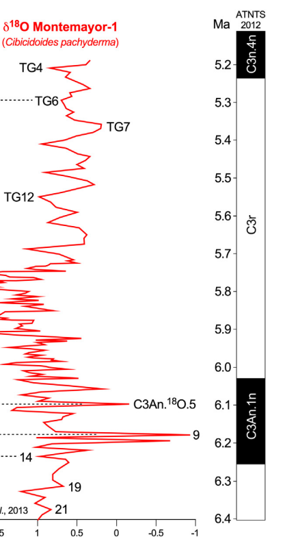
in parallel to the quantified mean annual in the Montemayor-1 hole directly calibrated S2012 refers to the Astronomically tuned
