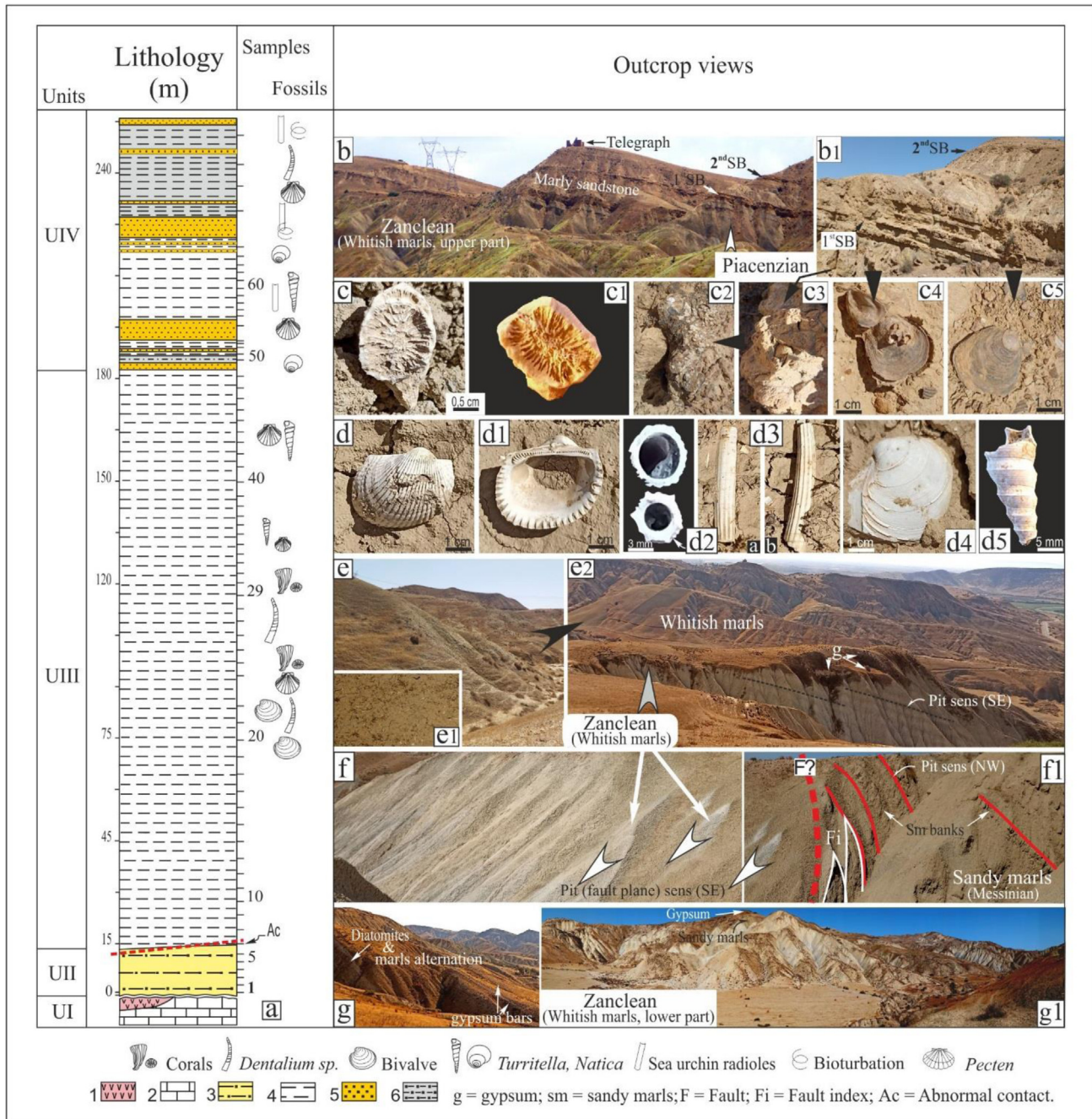
Fig. 7. Geological succession of the Sidi Brahim Telegraph section. Lithostratigraphic succession: 1: Gypsum; 2: Calcareous gypsum; 3: Sandy marls; 4: Blue (Whitish) marls; 5: Blue marls; 6: Sandstone; 7: Grey sandy marls. a: Lithology, samples and paleontological indications of the SBT geological section; b: Panoramic view showing the lithologic succession of the upper blue (whitish) marls (Zanclean) to the sandy marls and sandstone alternation (Piacenzian); b1: 1 st and 2 nd Sandstone bars (SB); c and c1: Scleractinian corals ( Ceratotrochus ( Edwardsotrochus ) pentaradiatus ); c2 and c3: Sandstone fossil concentration. c4 and c5: Ostreid shells of Hyotissa hyotis , fragments of Pectinids, colony of Balanus sp.; d and d1: Anadara diluvii shells. d and d3 (a,b): test of Dentalia sp. d4: Veneridae ( Pelecypora sp.); d5: Turritella sp. Note that fossils of figures c, c1, d, d1, d2, d3, d4 and d5 are of Zanclean age. e and e1: Blue (whitish) marls with dentals. e2: Panoramic view of the Blue (whitish) Zanclean marls: see gravity deposit (g: gypsum blocks), SE dip of the marl levels; f: Fault plane on marl sediments: see Blue (whitish) marl trails (white arrows) indicating fault plane pit; f1: Red lines indicate the plane of the sandy marl (sm) banks, broken line indicates hypothetical fault; g: Latest Messinian deposits (diatomite and marl alternation, gypsum); g1: Panoramic view showing the lower part of the Pliocene blue (whitish) marls.
