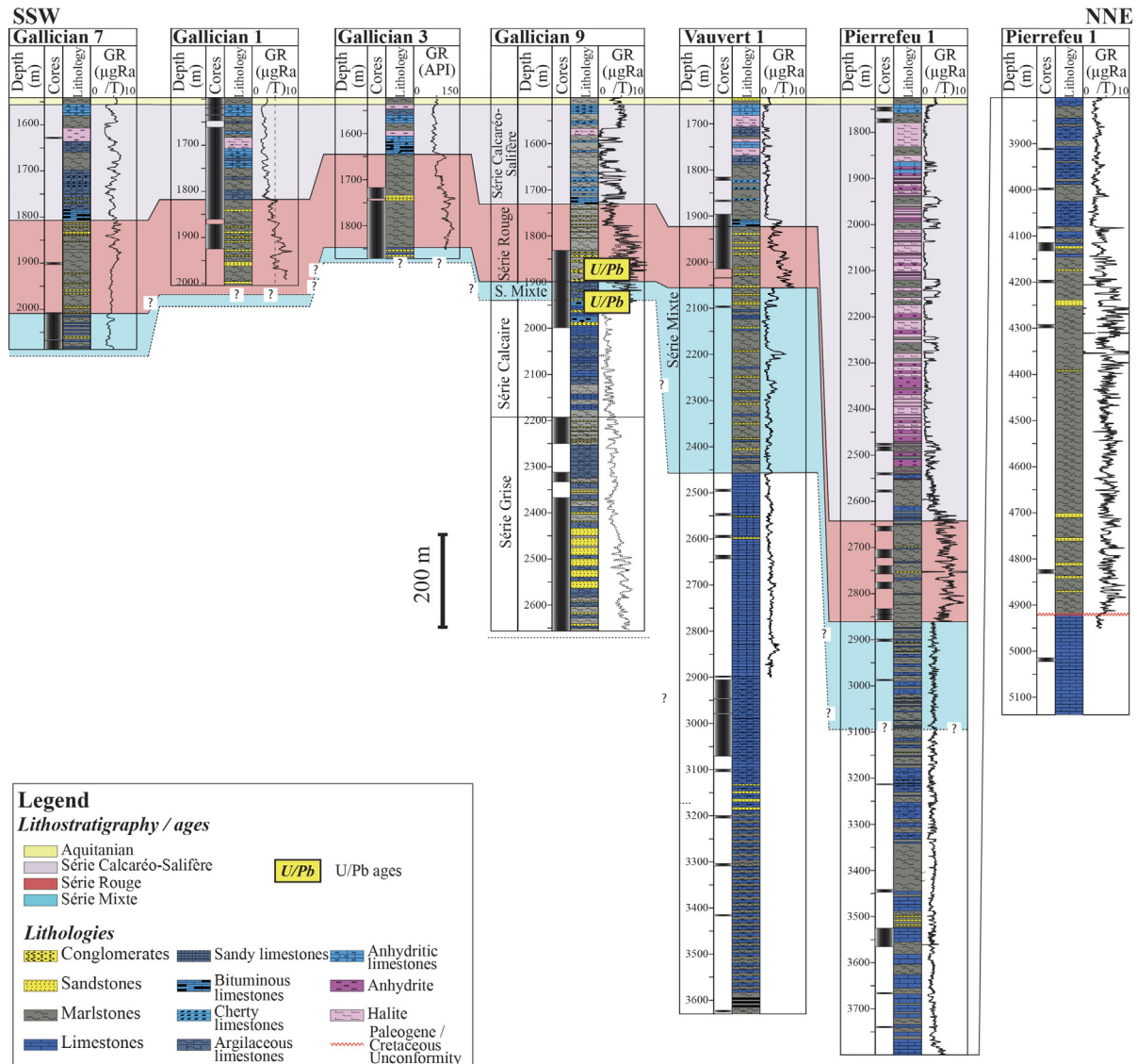
Fig. 4. Correlation panel of wells Gallician 7, Gallician 1, Gallician 3, Gallician 9, Vauvert 1 and Pierrefeu 1 from the Gallician and Pierrefeu sectors showing the sedimentary units, lithologies and lithostratigraphic correlations. Lithostratigraphic correlations are carried out using lithological similarities and gamma ray (GR) signal. \mu\text{gRa}/\text{T} : microgram of Radium/Time (radioactivity measurement).
