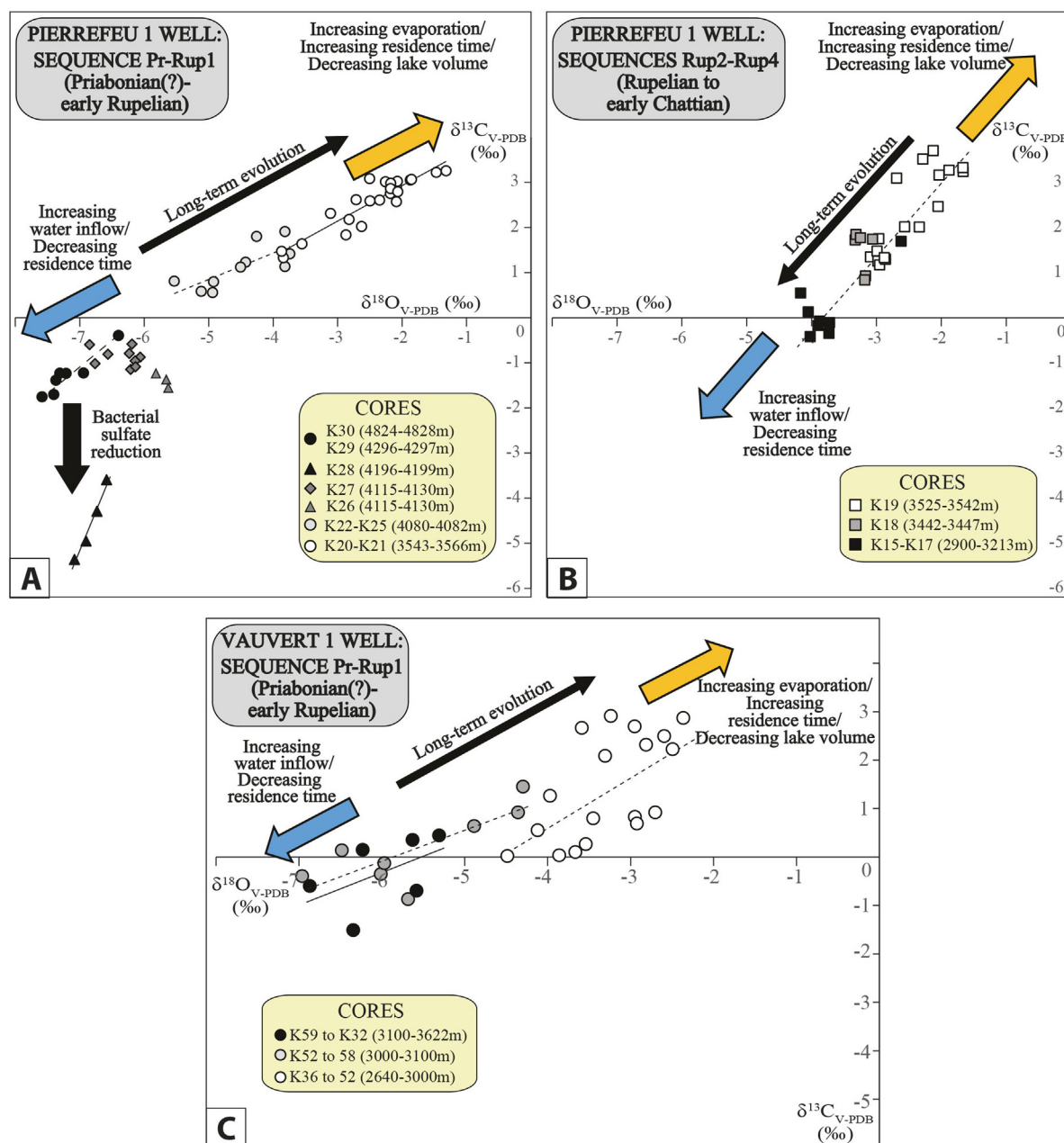
Fig. 13. \delta^{13}\text{C} and \delta^{18}\text{O} cross-plots of carbonates from Pierrefeu 1 well (A, B) and Vauvert 1 well (C) within the “Série Grise” Formation.
