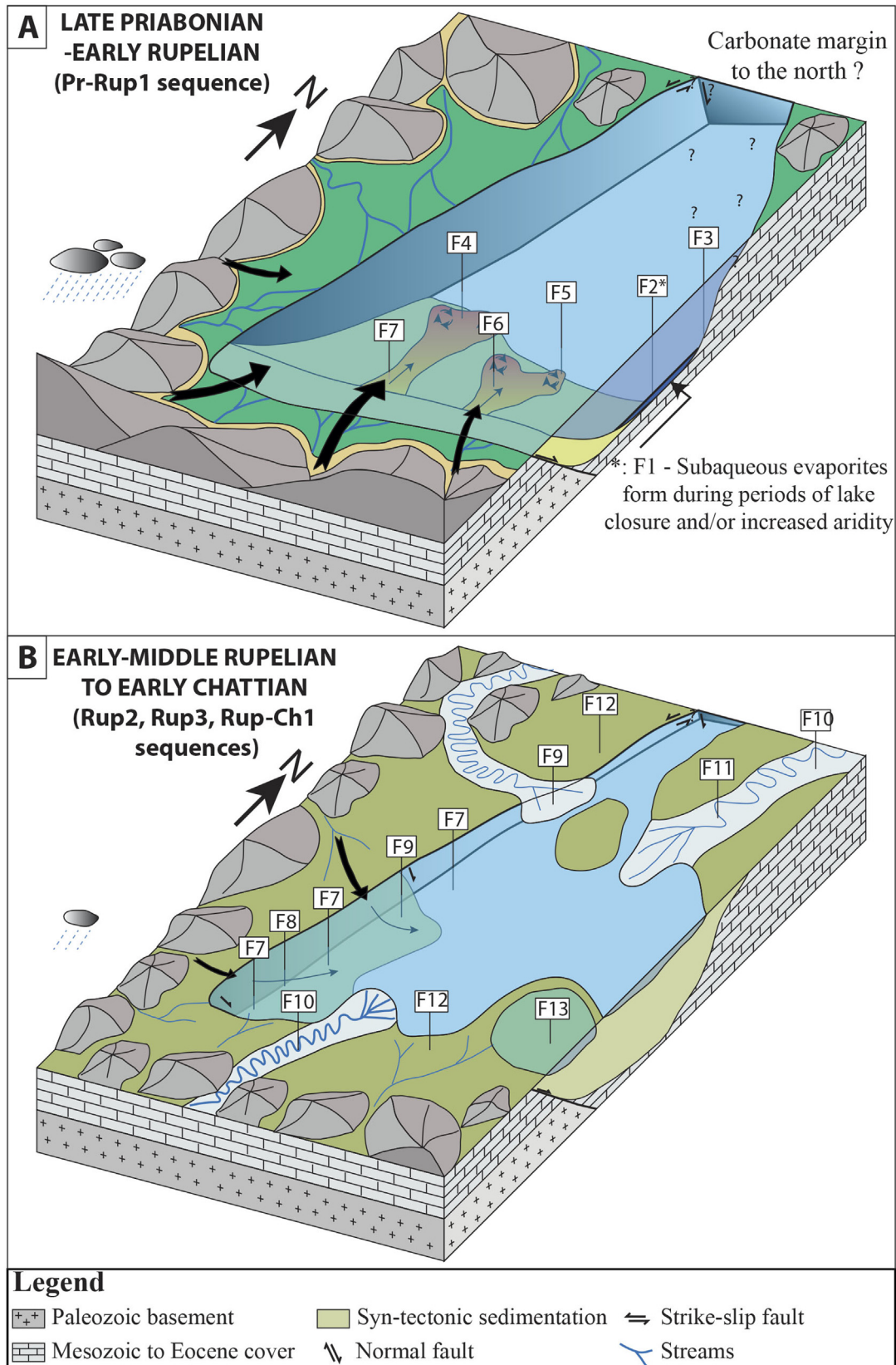
Fig. 15. Simplified block diagrams showing the depositional models for (A) profundal perennial lake, and (B) shallow lake with extensive floodplain. Evaporites (F1 facies) formed within perennial lake conditions precipitate in compartmentalized areas with maximum reduction of connection to the main saline waterbody (see Fig. 16 for further details).
