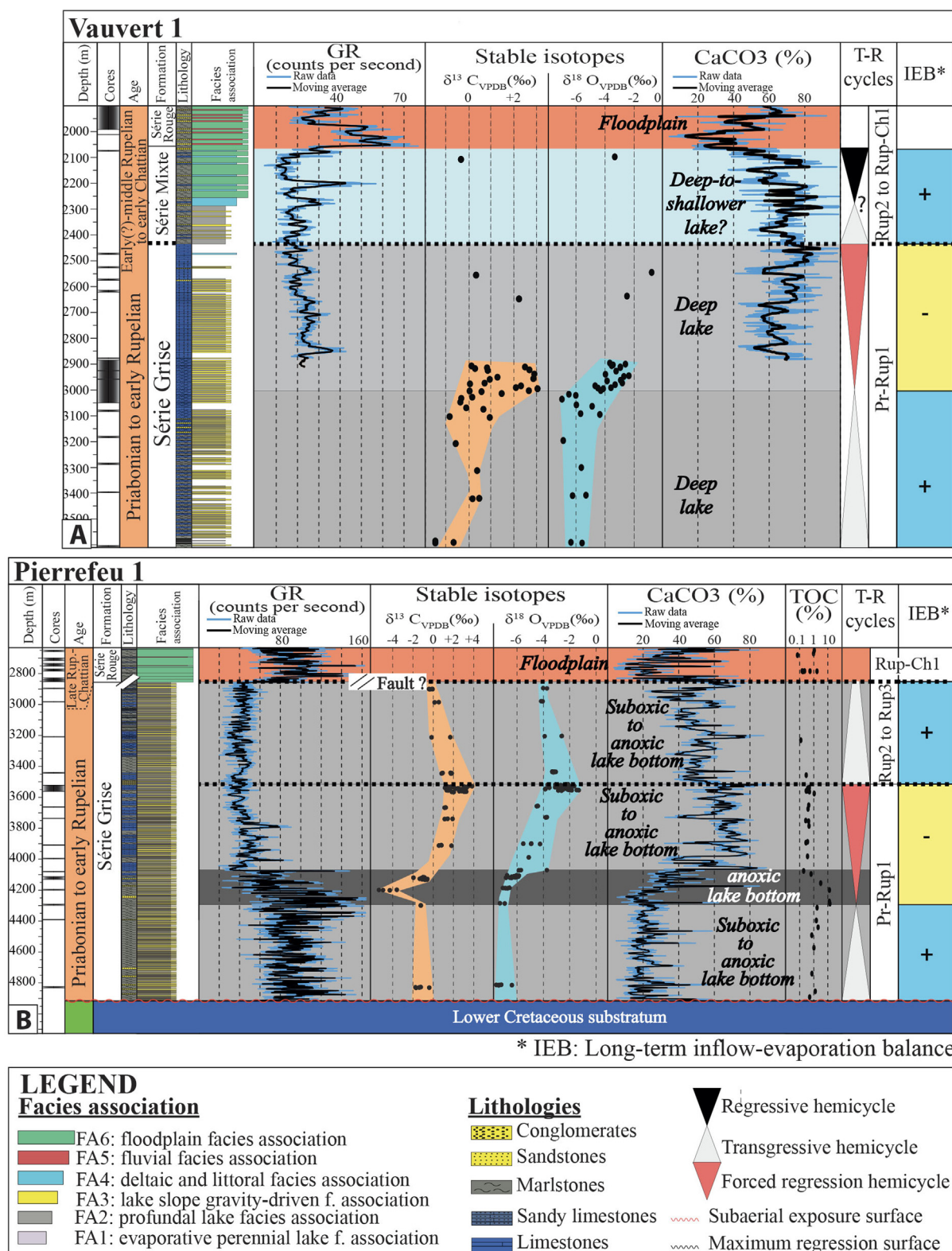
Fig. 14. Synthetic panel of vertical variations in \delta^{18}\text{O} , \delta^{13}\text{C} , \text{CaCO}_3 content, Gamma Ray signal, TOC (Total Organic Carbon), and the interpreted lacustrine transgressive and regressive trends and long-term inflow-evaporation balance: A: Vauvert 1 well; B: Pierrefeuf 1 well.
