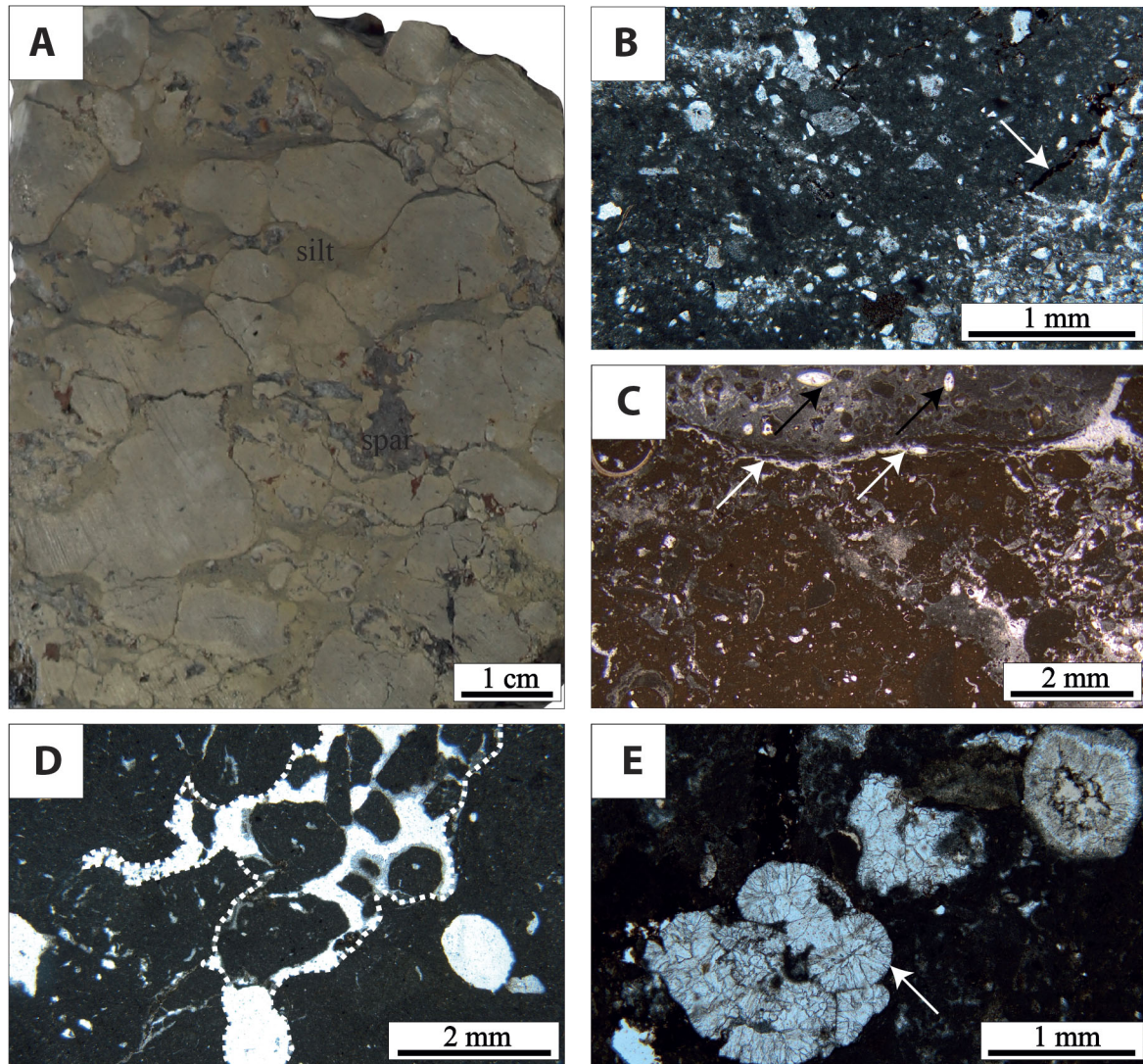
Fig. 11. Brecciated and palustrine limestones (F13 facies). (A) Core photograph of a nodular limestone (F13 facies). The nodules (glauconites) are well differentiated indicating long-duration pedogenic processes, the voids between the nodules are filled with silt and blocky calcite (spar). (B) Thin section of a pedogenically modified calcarenite (F7 facies) displaying cracks lined with the clay material (white arrow). This facies is frequent at the top of the F7 calcarenite beds. (C) Thin section of an intraclastic limestone with microbial crusts (F9 facies) displaying subaerial exposure features (silt fill, perigranular cracks (white arrows) around a nodule composed of ostracodal mudstone (black arrows indicate ostracods). (D) Microphotograph showing a conduit (outlined by the dashed line) within a dense dark micrite filled with clasts of the same micrite, resulting probably from the enlargement of a root cavity and filled with glauconites (PPL). (E) Thin section of a palustrine carbonate made of dense dark micrite and showing a well-developed cluster of Microcodium .
