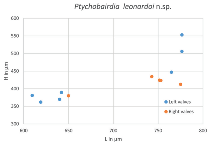
Fig. 6. Height (H)/length (L) diagram for Ptychobairdia leonardoii n.sp. In blue: left valves; in red: right valves.
